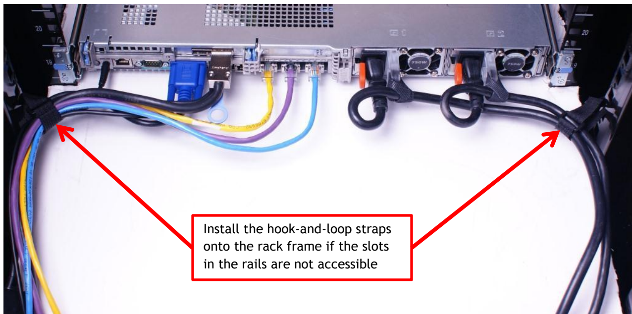
Figure 11. Cabling a system installed in static rails
