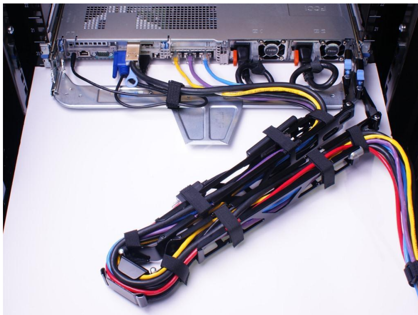
Figure 6. Right-side mounted CMA installation (CMA shown in service position)
